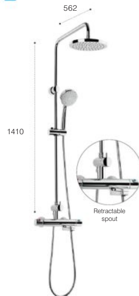
4. Wall-mounted thermostatic shower column with kit
