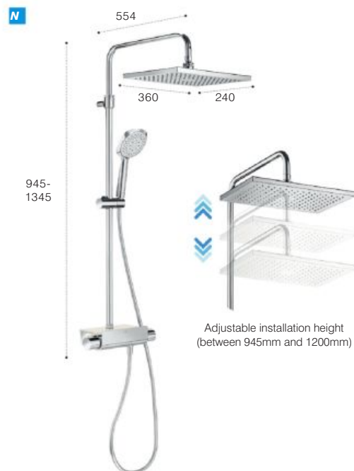
2. Thermostatic shower column with adjustable installation height and swivelling rain shower head
