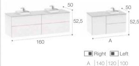
Base unit for in countertop basins
