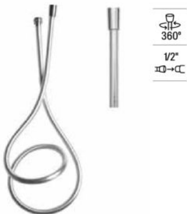
Satin PVC flexible shower hose Satin PVC 1.50 m anti-torsion universal flexible shower hose. 1/2". A5B2016C00 A5B2116C00 A5B2216C00
